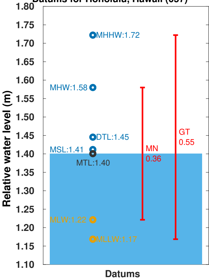
Datums for Honolulu, Hawaii (057)
